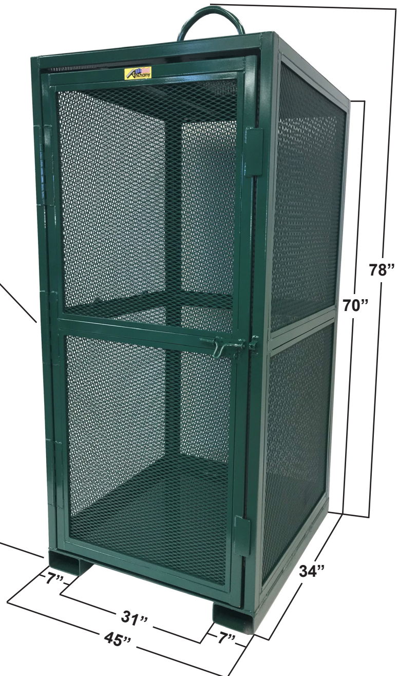
FORKLIFT POCKETS
