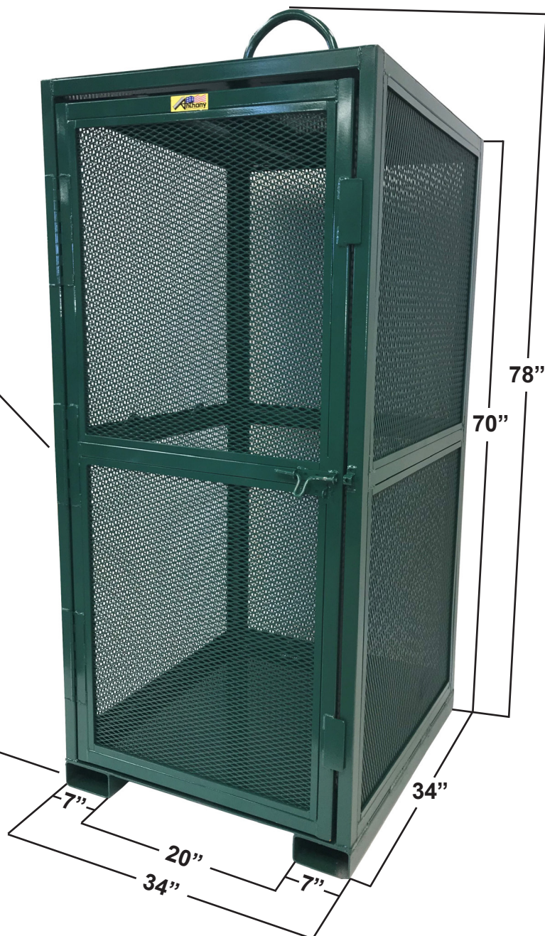
FORKLIFT POCKETS
